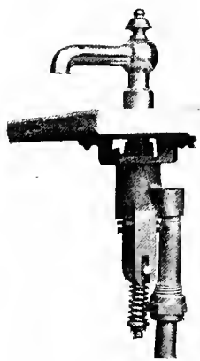
Fig. 3548. SWING-NOZZLE FAUCET.
